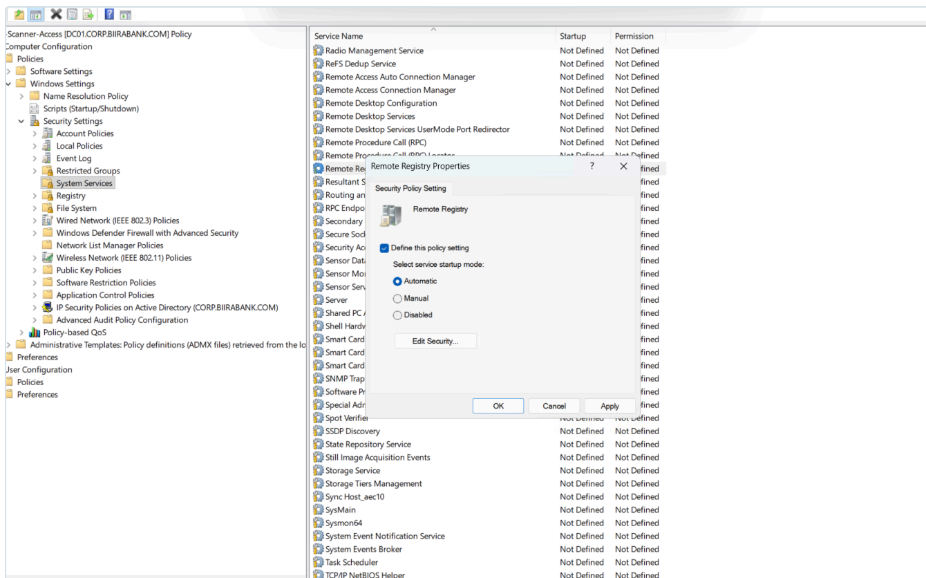
Figure 19.44: Computer Configuration, Windows Settings, Security Settings, System Services. The service is defined by policy rather than set by hand on each machine, which is the difference between a configuration and a control ( CM-6 ).
