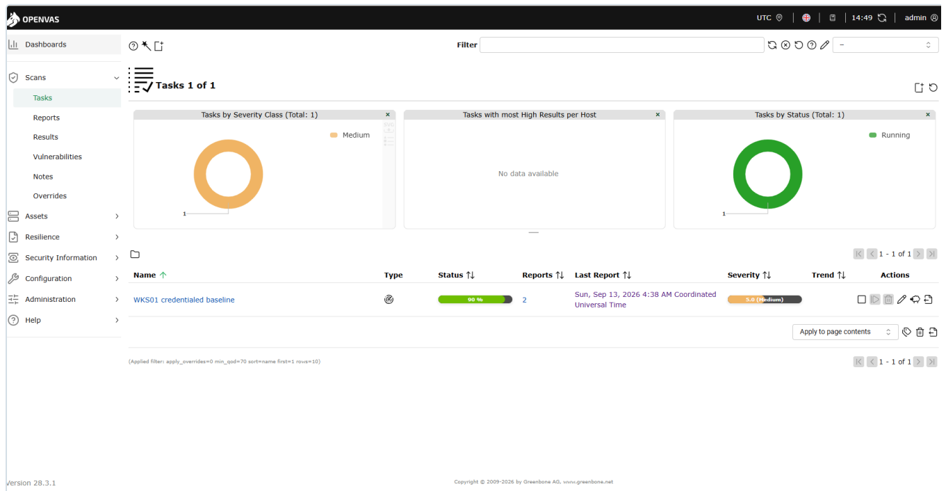
Figure 19.48: The WKS01 credentialed baseline task in Greenbone, in progress. The name matters: this run is the reference the next one is compared against, which is what makes a remediation loop possible rather than a one-off report.
