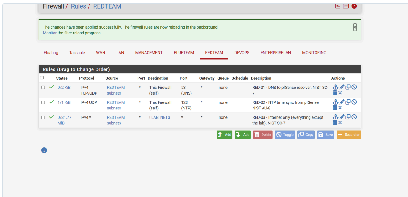
Figure 13.13: The REDTEAM interface after the legacy any-to-any rule was deleted. Three rules, each carrying its identifier, justification and control mapping. Compare Figure 13.8, where the disabled permit-all was still present.
