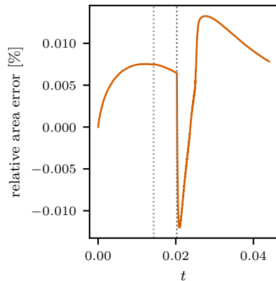
(c) merged-area conservation
