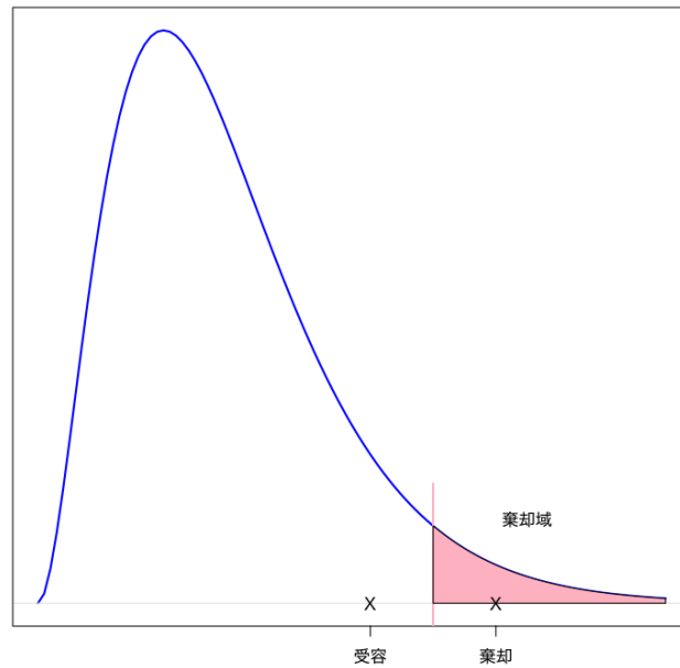
Figure 2: 棄却と受容
