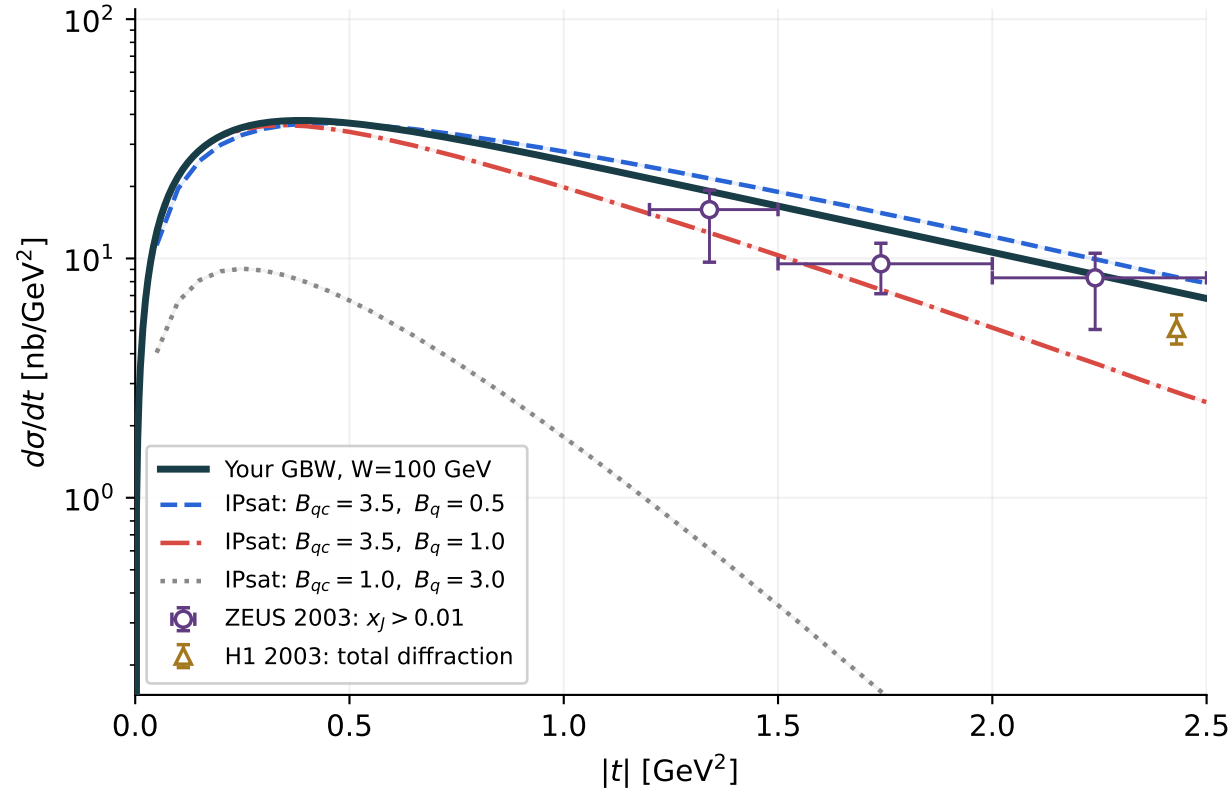
Figure 1 comparison: W = 100 GeV
