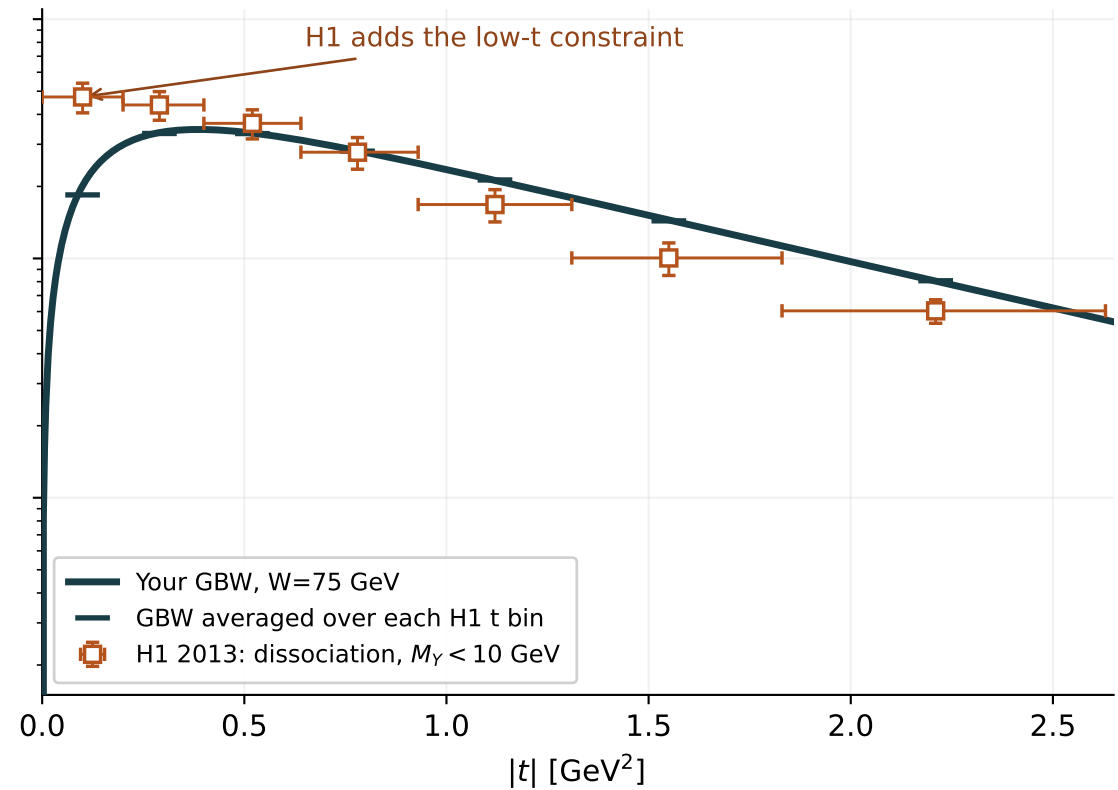
H1 data reaching small |t| : W = 75 GeV
