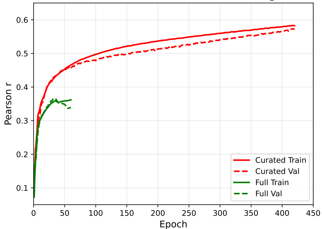
B. Train vs Validation: No Overfitting
