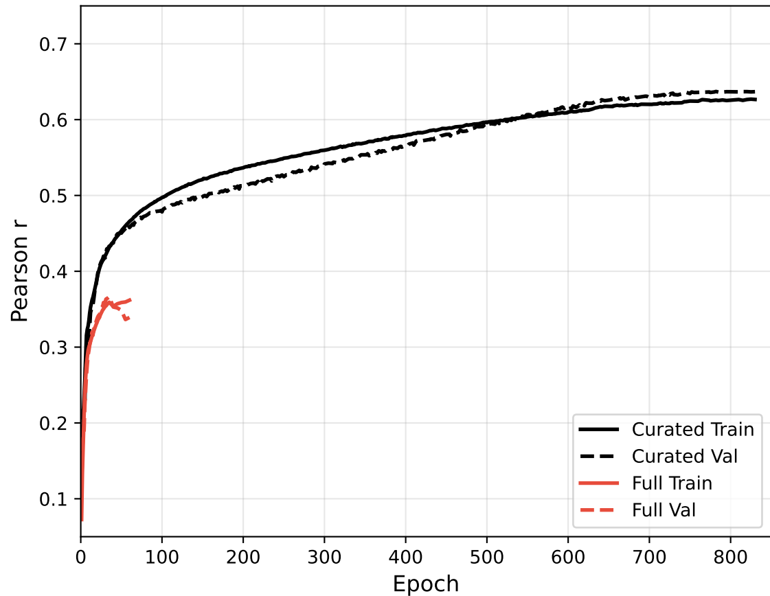
B. Train vs Validation: No Overfitting
