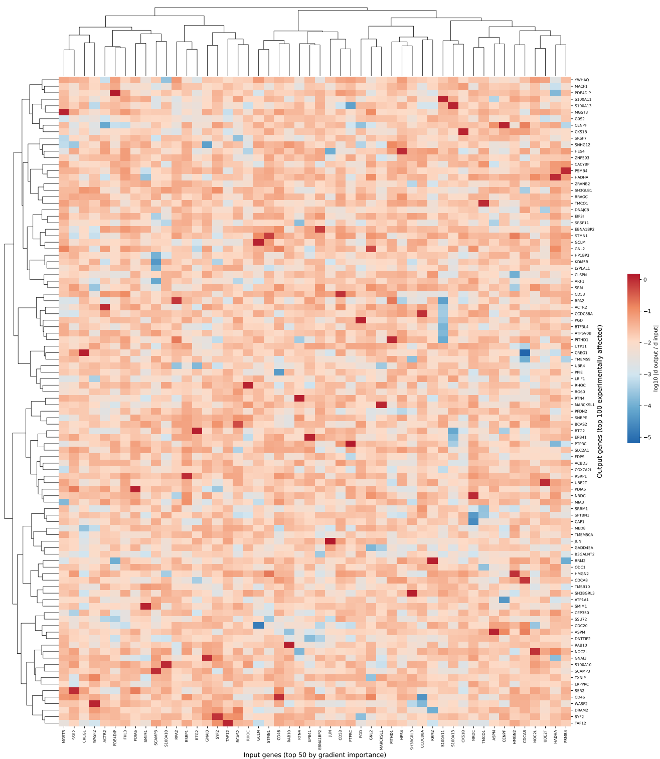
Jacobian Regulatory Map: TFRC Perturbation ( |d \text{ output} / d \text{ input}| at NTC baseline)
