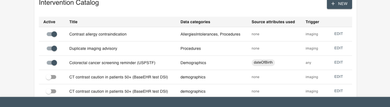
Figure 9.1: Decision Support Interventions - Configuration Interface
