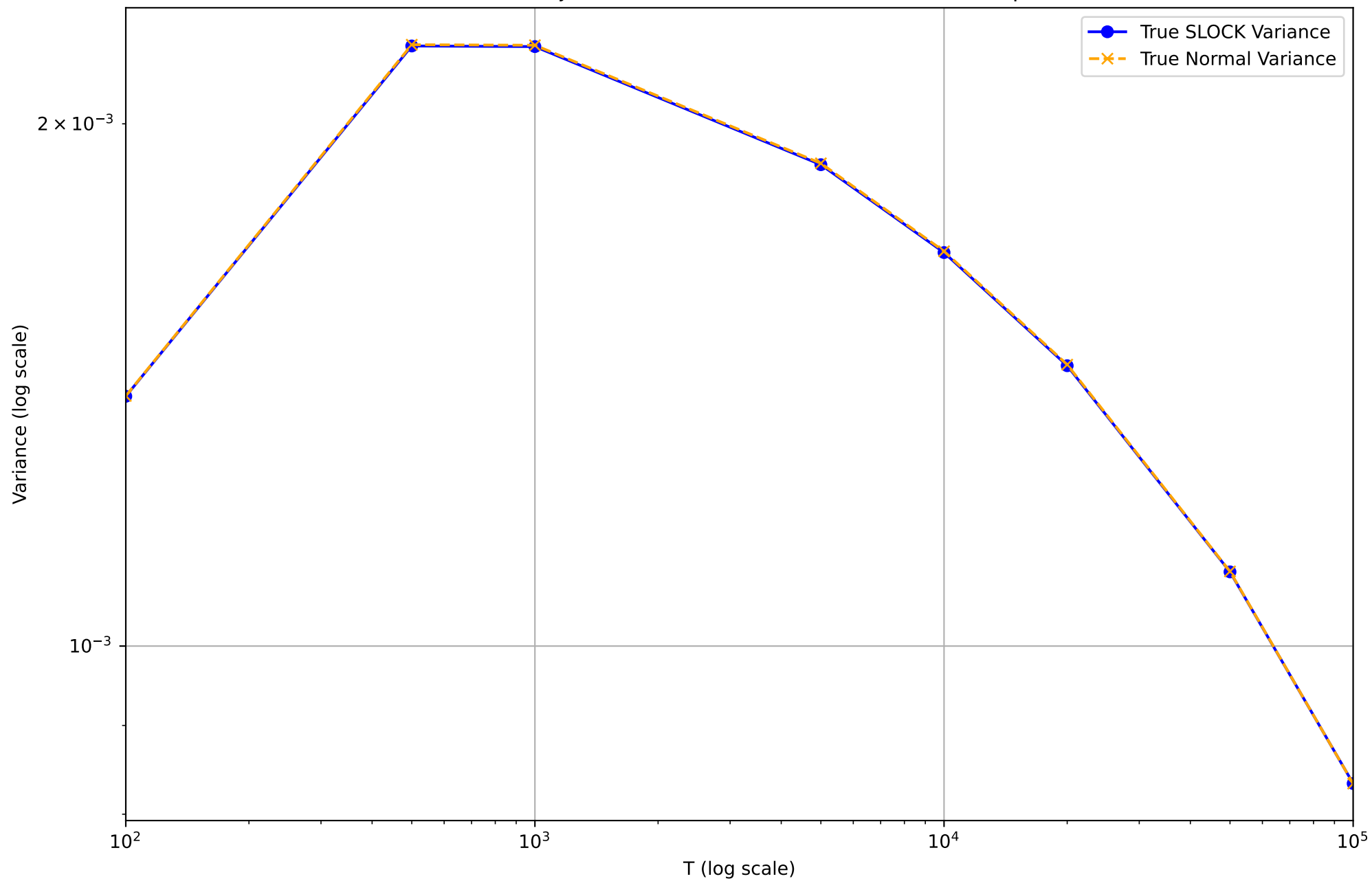
True Variance Trajectories (SLOCK vs Normal) eta=0.01, alpha=1.3
