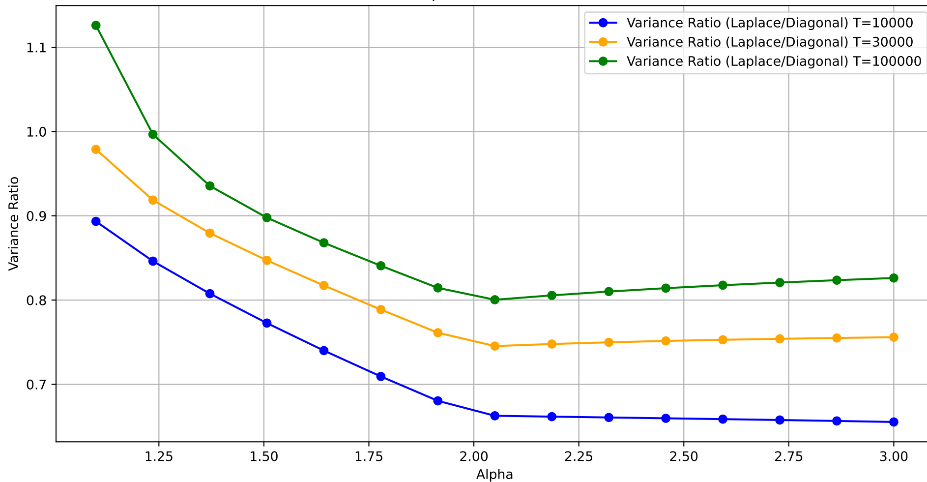
Corrected Variance Ratio of Laplace approximation to Diagonal approximation for linear schedule at K=1 for different alpha values, beta=1.2, Delta=1
