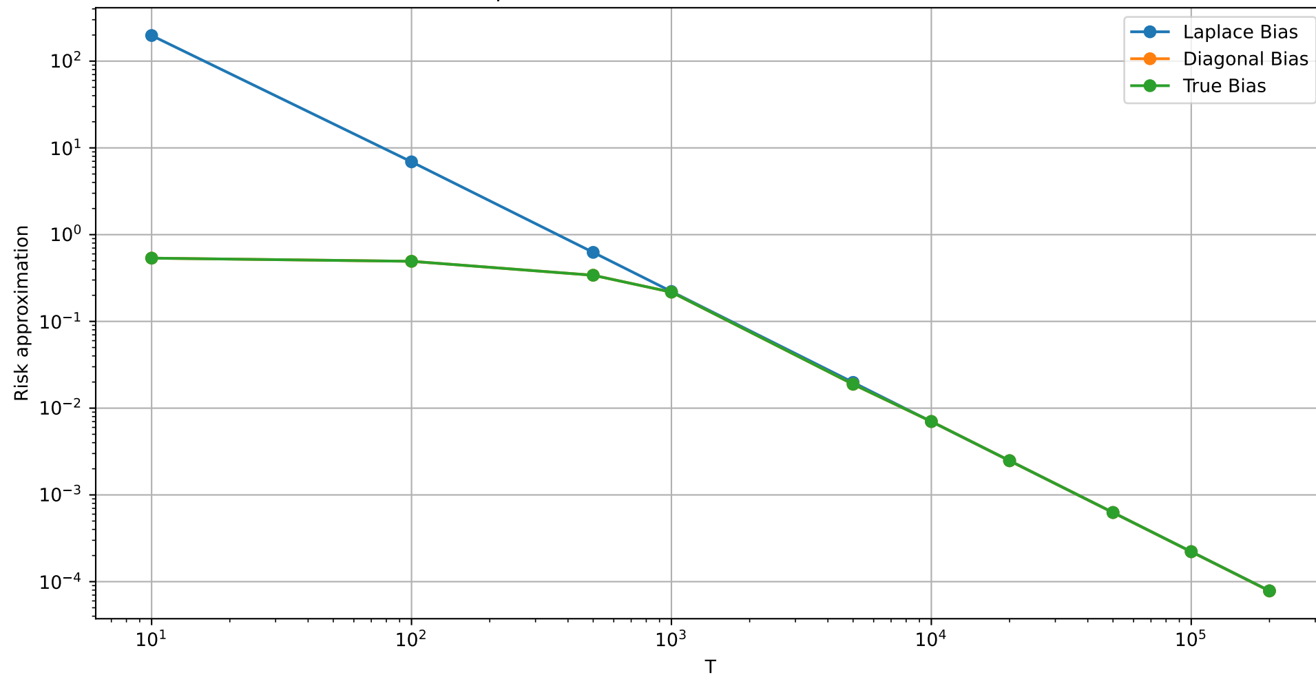
Bias components of Laplace approximation vs Diagonal approximation for linear schedule \alpha=2 , \beta=2 , T_{\max}=200000 , K=t/T=1
