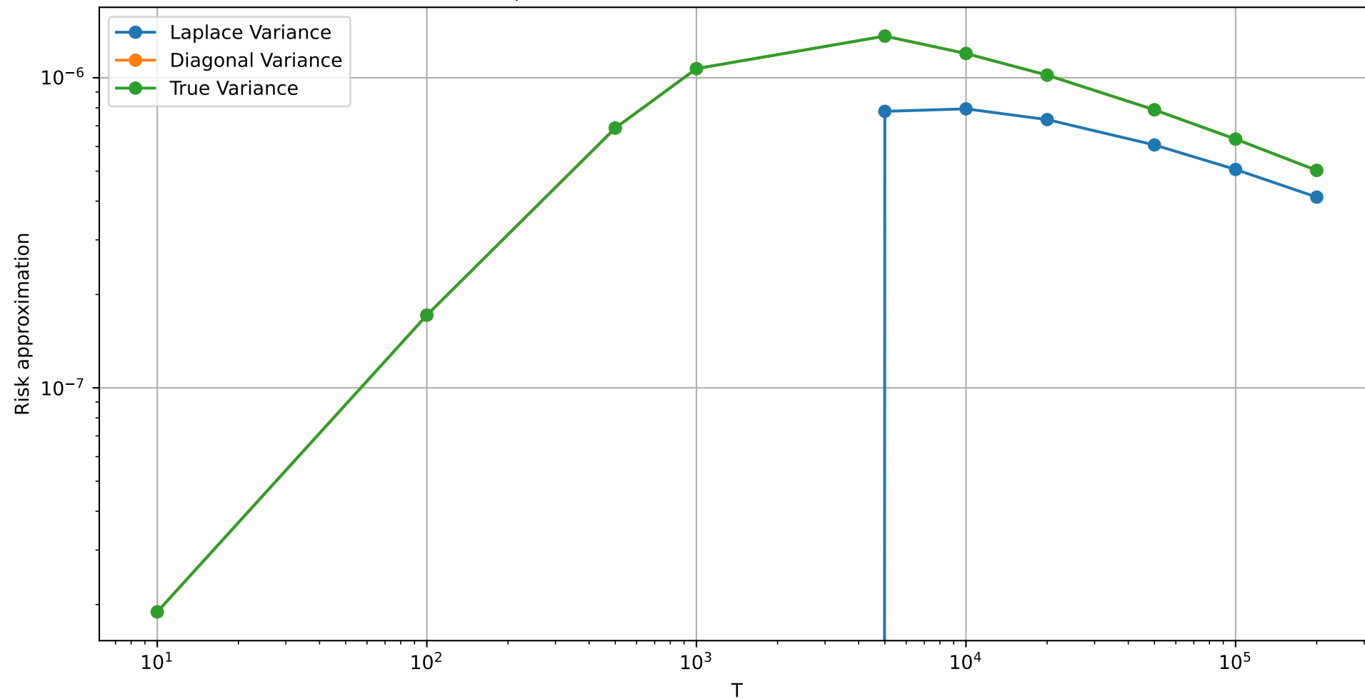
Variance components of Laplace approximation vs Diagonal approximation for linear schedule \alpha=2 , \beta=2 , T_{\max}=200000 , K=t/T=1
