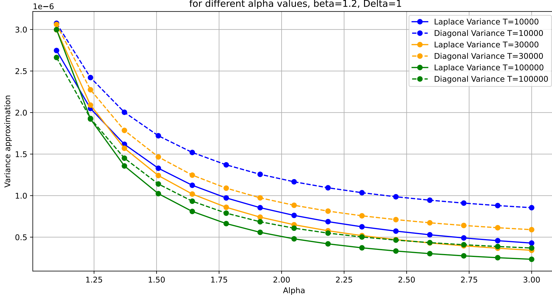
Variance of Laplace approximation vs Diagonal approximation for linear schedule at K=1 for different alpha values, beta=1.2, Delta=1
