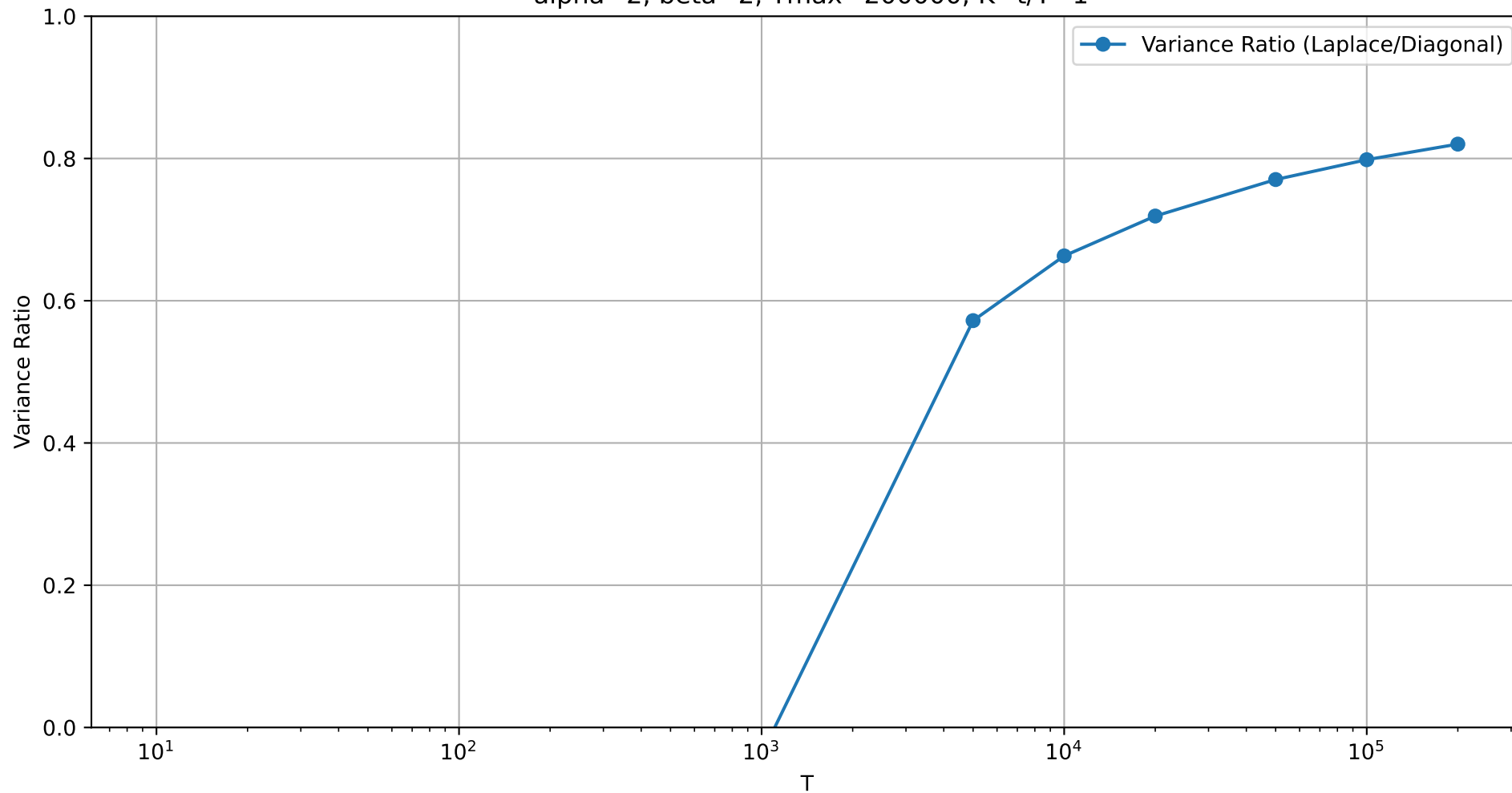
Variance Ratio of Laplace approximation to Diagonal approximation for linear schedule \alpha=2 , \beta=2 , T_{\max}=200000 , K=t/T=1
