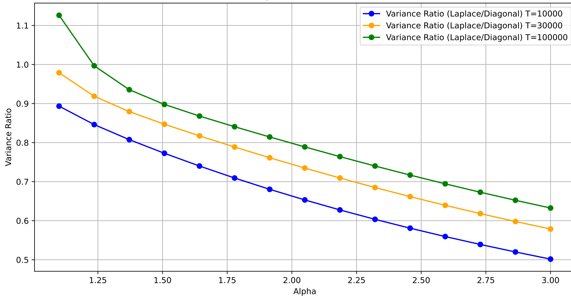
Variance Ratio of Laplace approximation to Diagonal approximation for linear schedule at K=1 for different alpha values, beta=1.2, Delta=1
