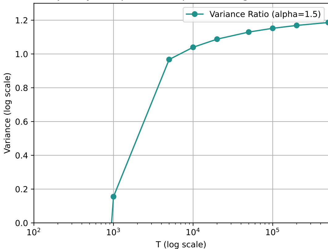
Variance Trajectory for \alpha=1.5 (Laplace vs Diagonal) for WSD schedule
