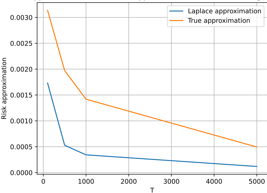
Linear schedule: Laplace risk approximation vs True risk approximation for different T, sigma=0.1,
