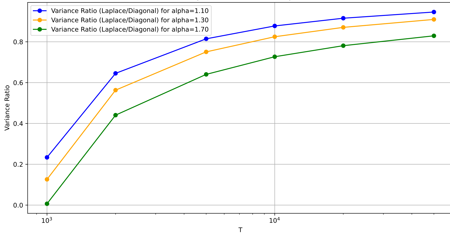
Variance Ratio Trajectories for Different Alphas, dim=1000
