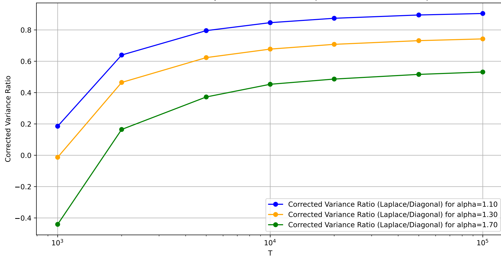
Corrected Variance Ratio Trajectories for Different Alphas, \text{dim}=(Tb100)^{**}(1b\alpha)
