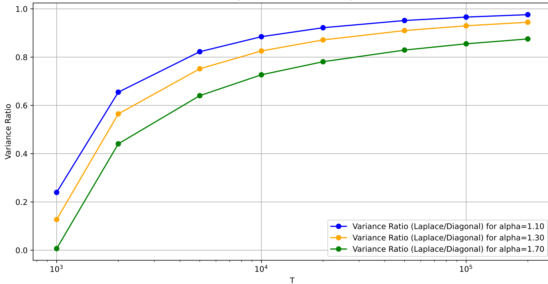
Variance Ratio Trajectories for Different Alphas, dim=0.02T
