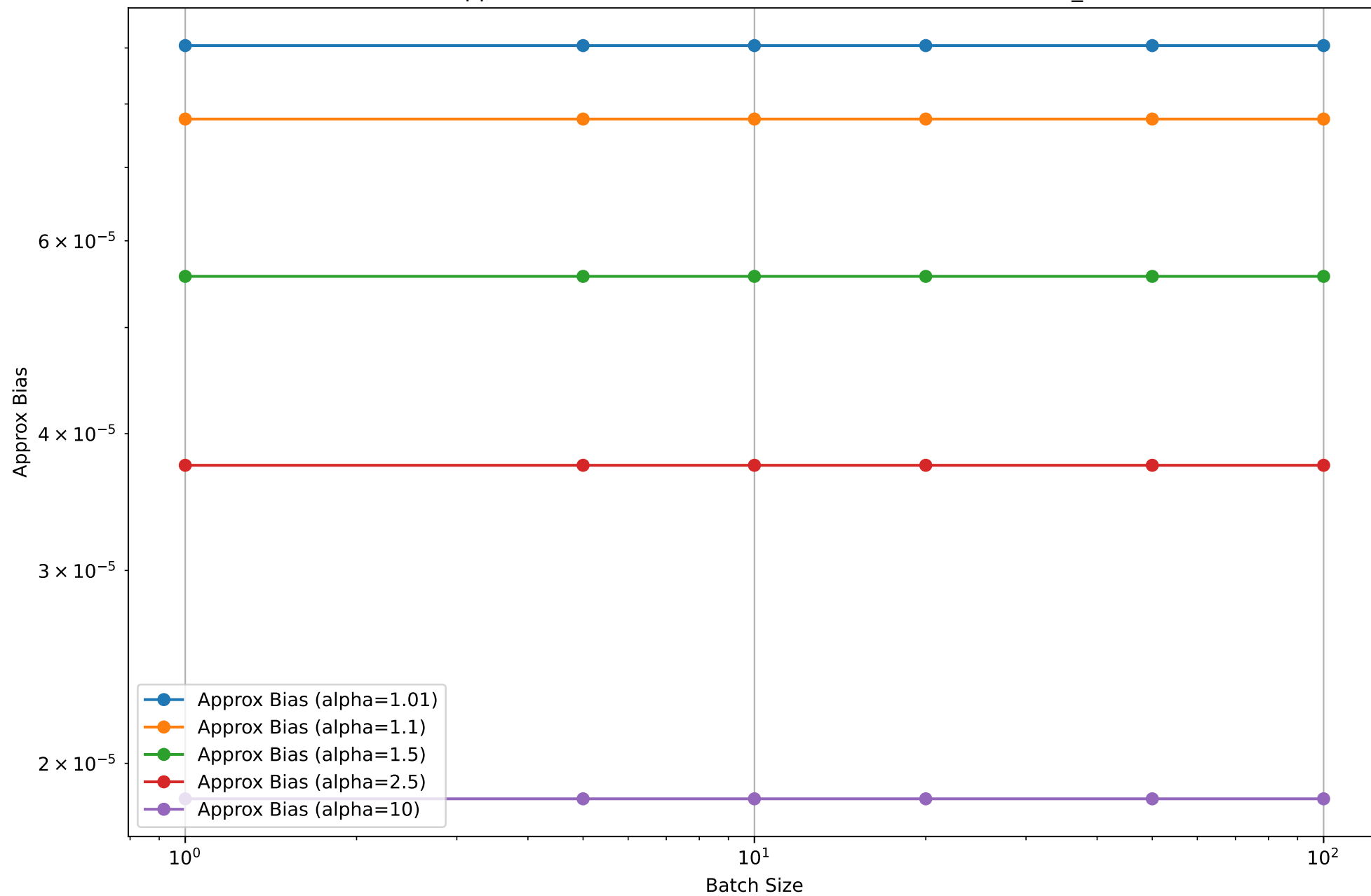
Slock Approx Bias for Different Batch Sizes; b \cdot T = 200000 , \eta_{\text{star}}
