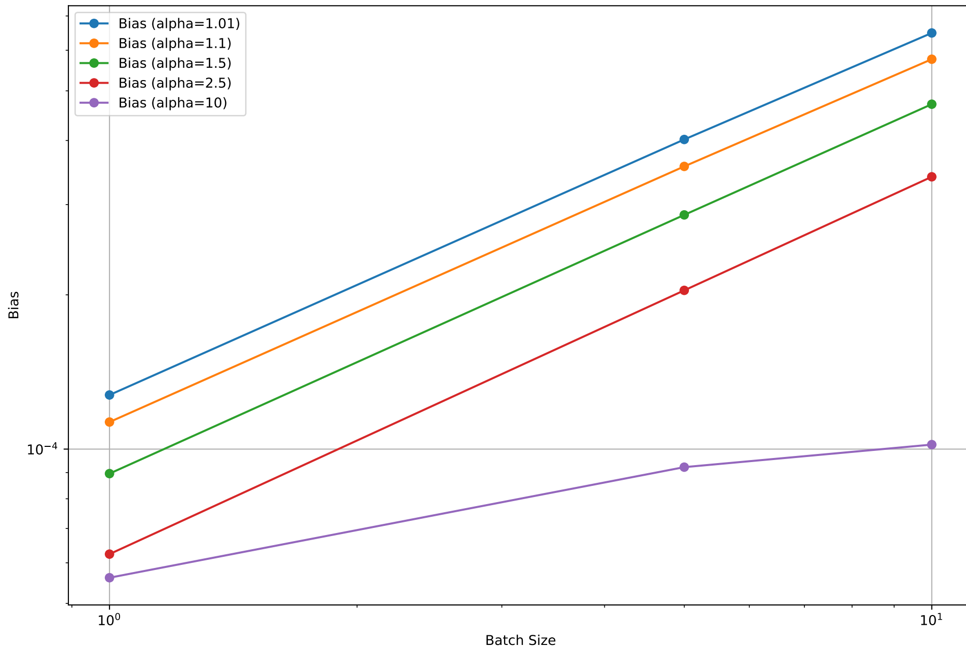
Slock Bias for Different Batch Sizes; b \cdot T = 100000 , \eta fixed at 0.01
