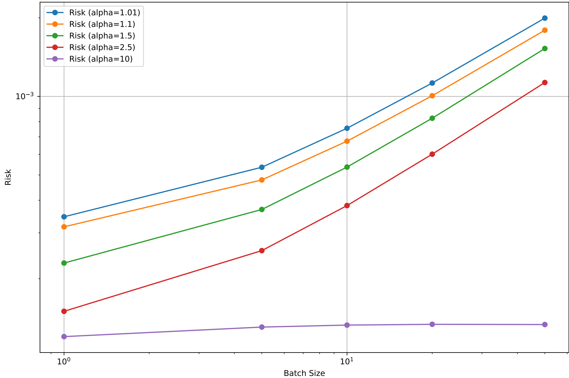
Slock Risk for Different Batch Sizes; b \cdot T = 100000 , \eta_{\text{star}}
