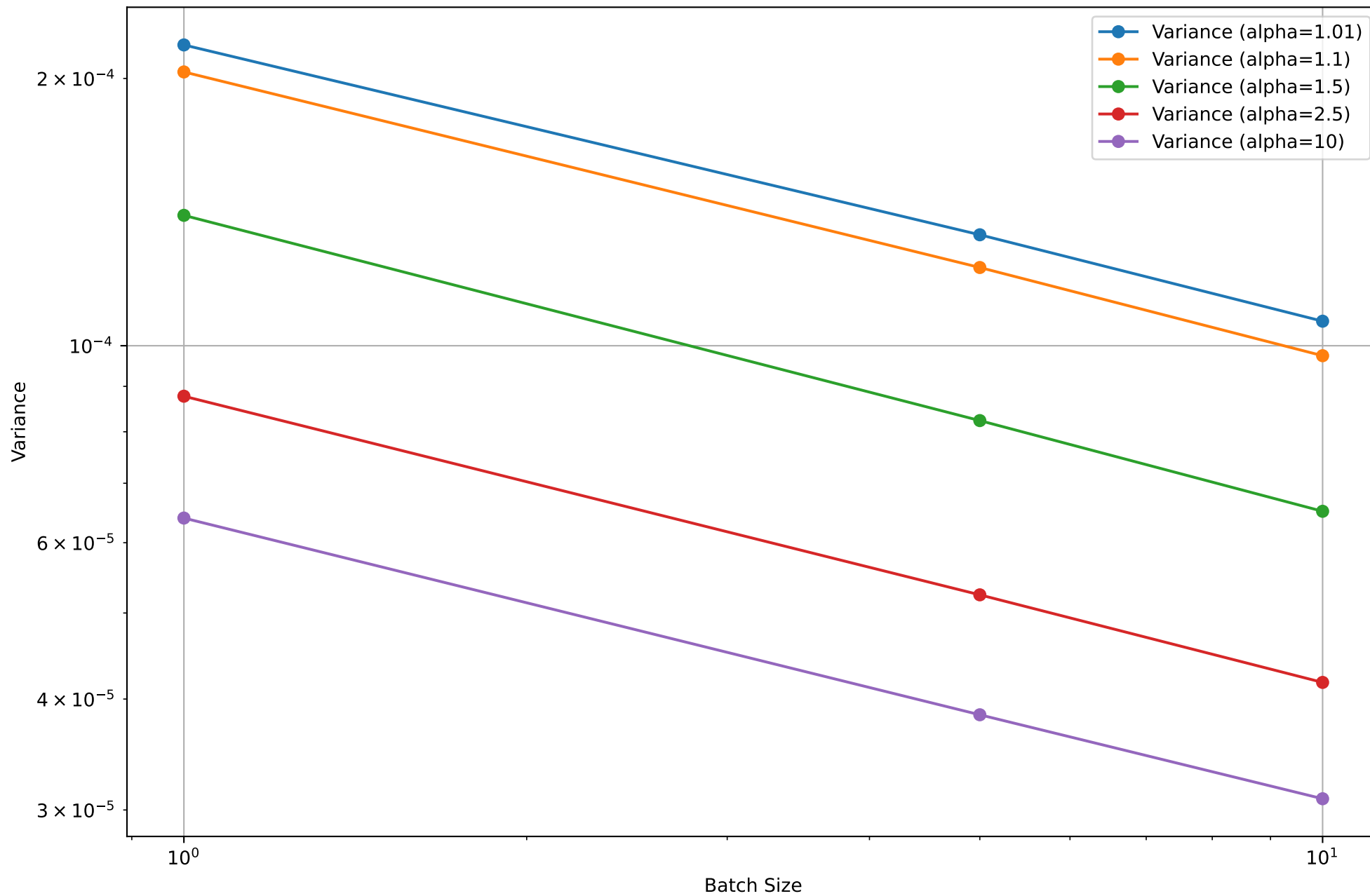
Slock Variance for Different Batch Sizes; b \cdot T = 100000 , \eta fixed at 0.01
