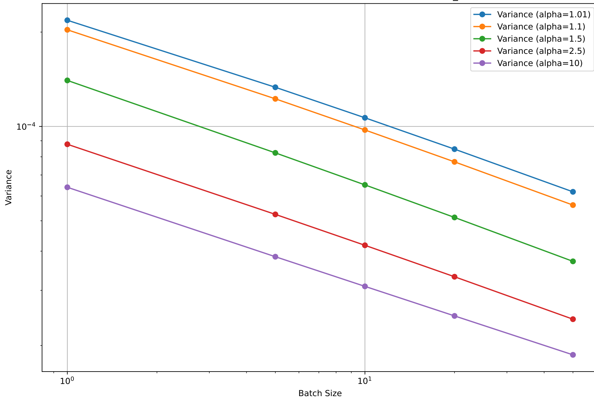
Slock Variance for Different Batch Sizes; b \cdot T = 100000 , \eta_{\text{star}}
