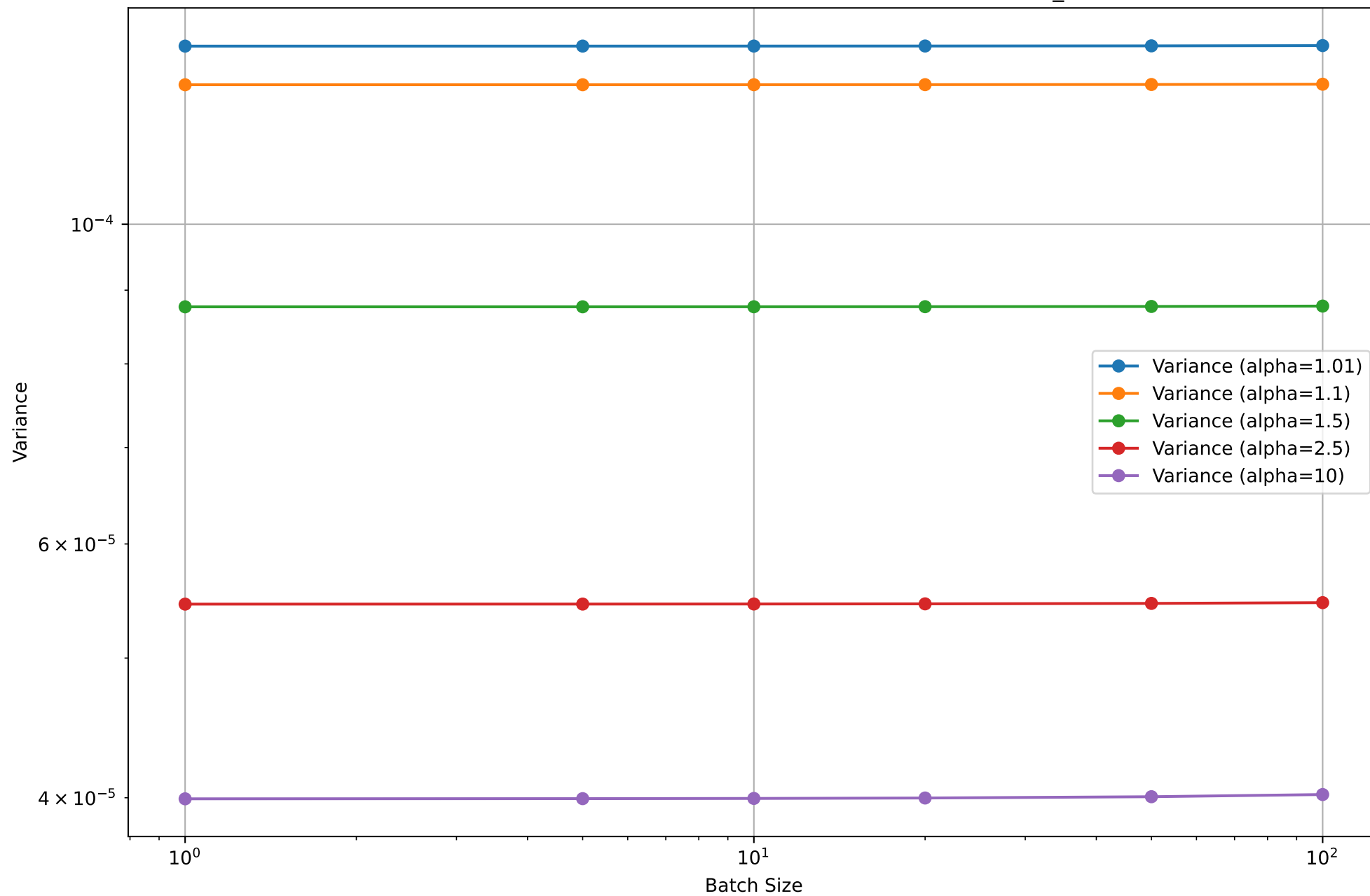
Slock Variance for Different Batch Sizes; b \cdot T = 200000 , \eta_{\text{star}}
