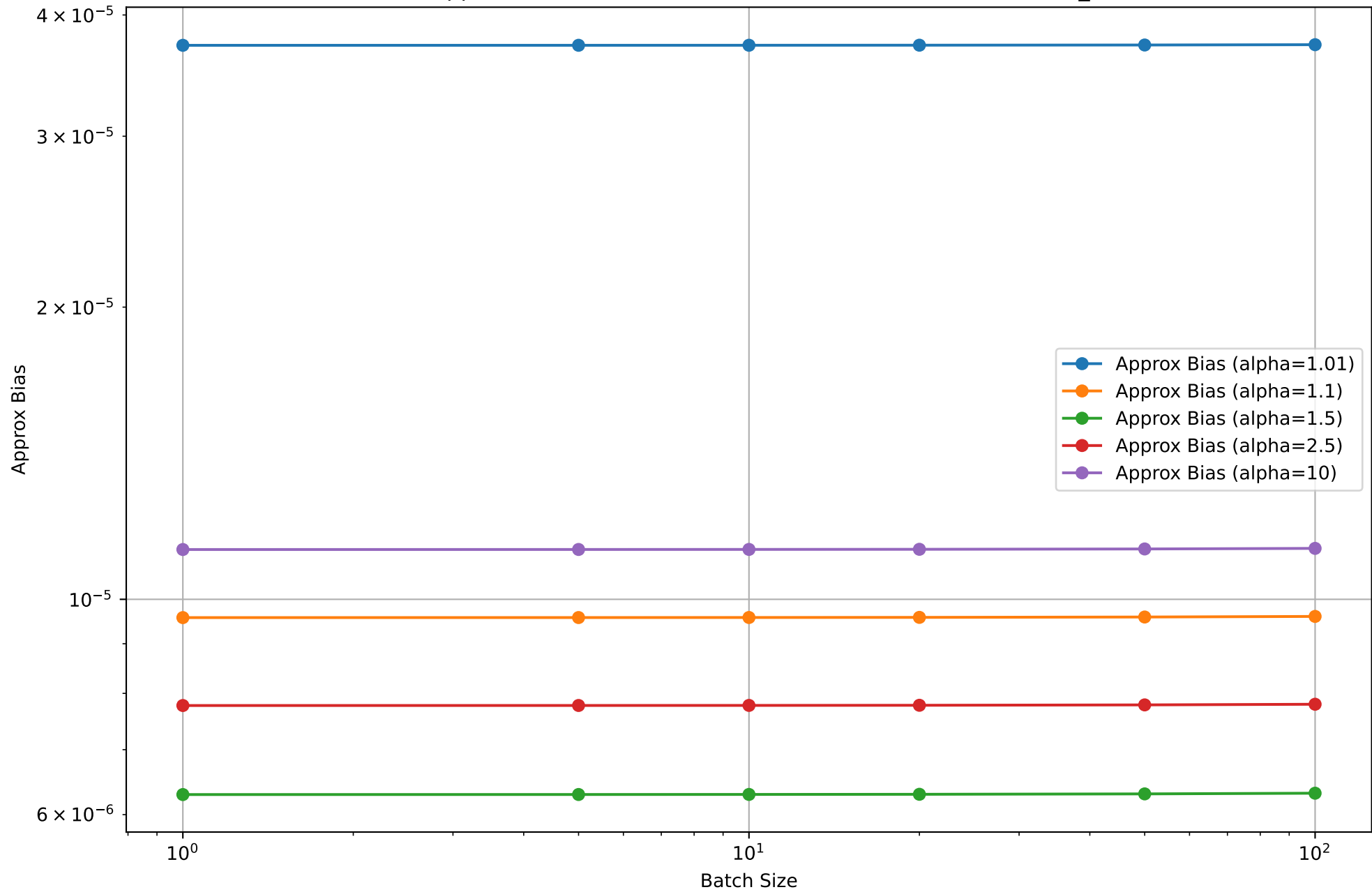
Slock Approx Bias for Different Batch Sizes; b \cdot T = 20000000 , \eta_{\text{star}}
