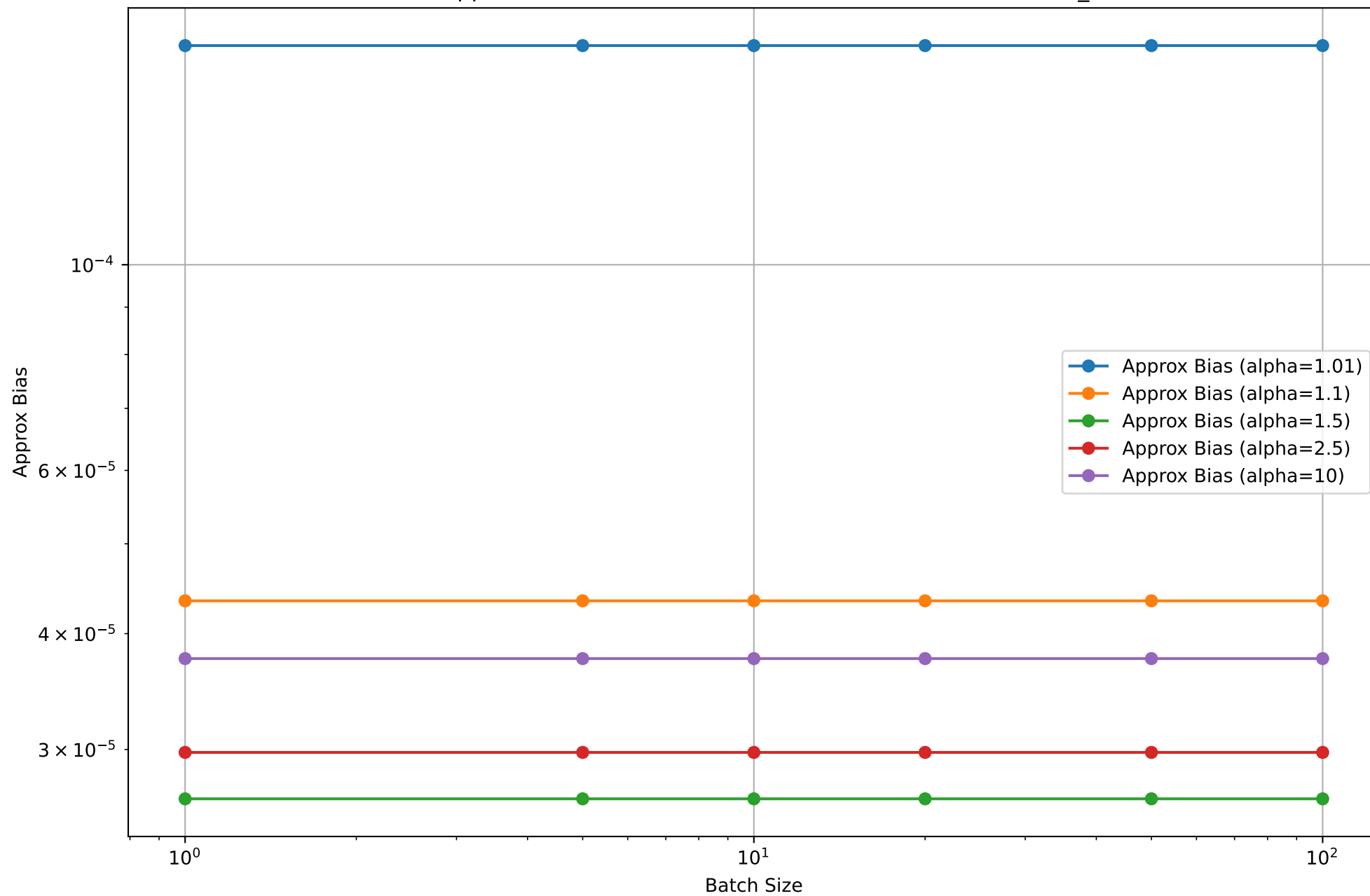
Slock Approx Bias for Different Batch Sizes; b \cdot T = 2000000 , \eta_{\text{star}}
