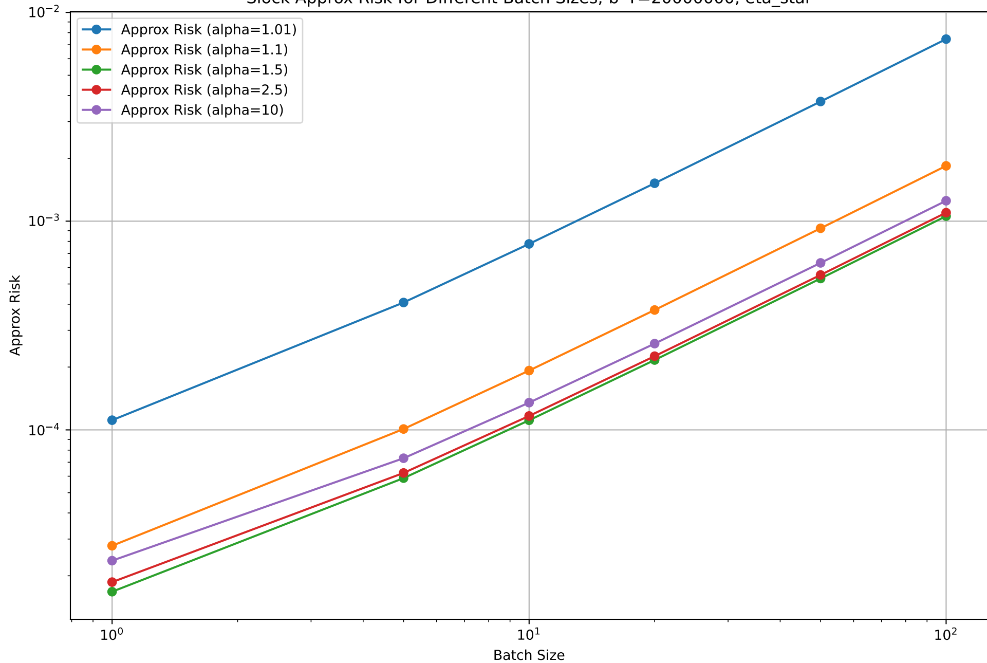
Slock Approx Risk for Different Batch Sizes; b \cdot T = 20000000 , \eta_{\text{star}}
