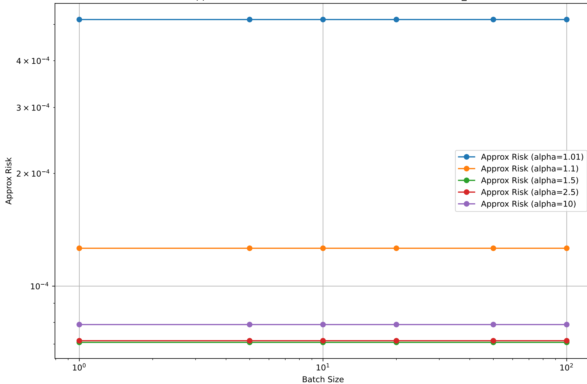
Slock Approx Risk for Different Batch Sizes; b \cdot T = 2000000 , \eta_{\text{star}}
