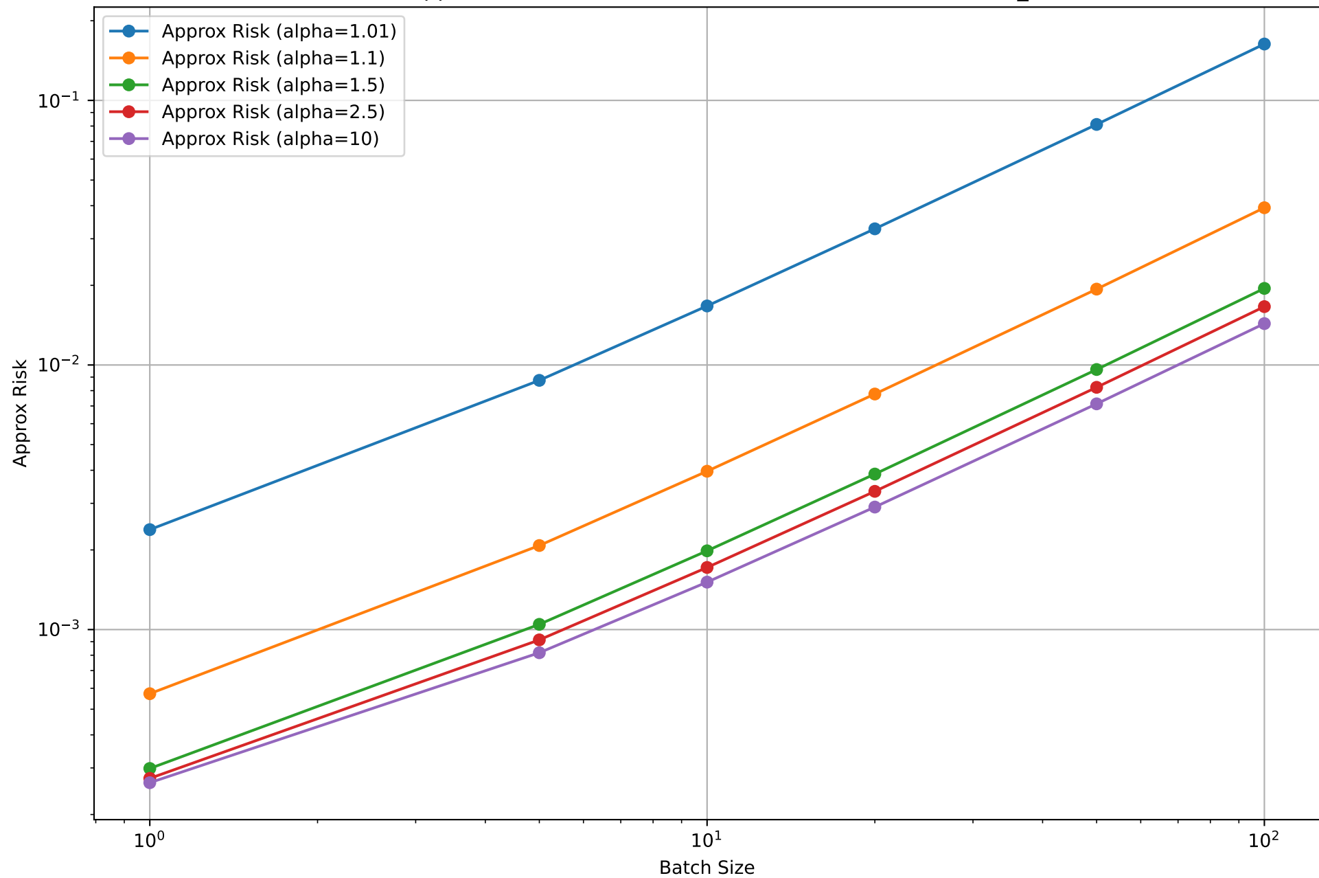
Slock Approx Risk for Different Batch Sizes; b \cdot T = 200000 , \eta_{\text{star}}
