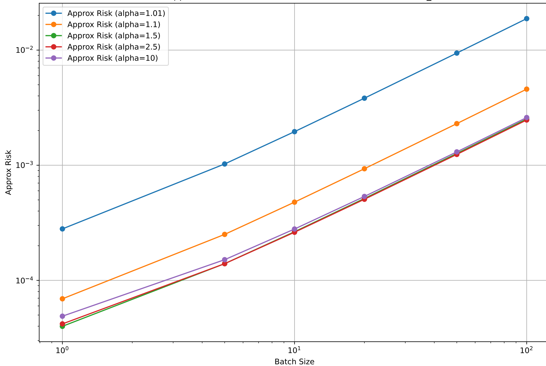
Slock Approx Risk for Different Batch Sizes; b \cdot T = 5000000 , \eta_{\text{star}}
