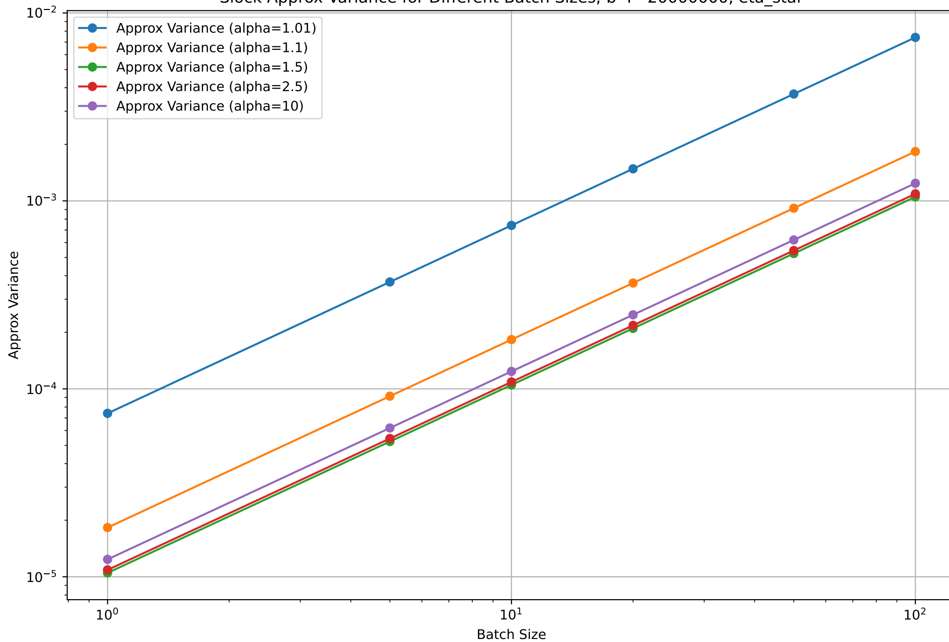
Slock Approx Variance for Different Batch Sizes; b \cdot T = 20000000 , \eta_{\text{star}}
