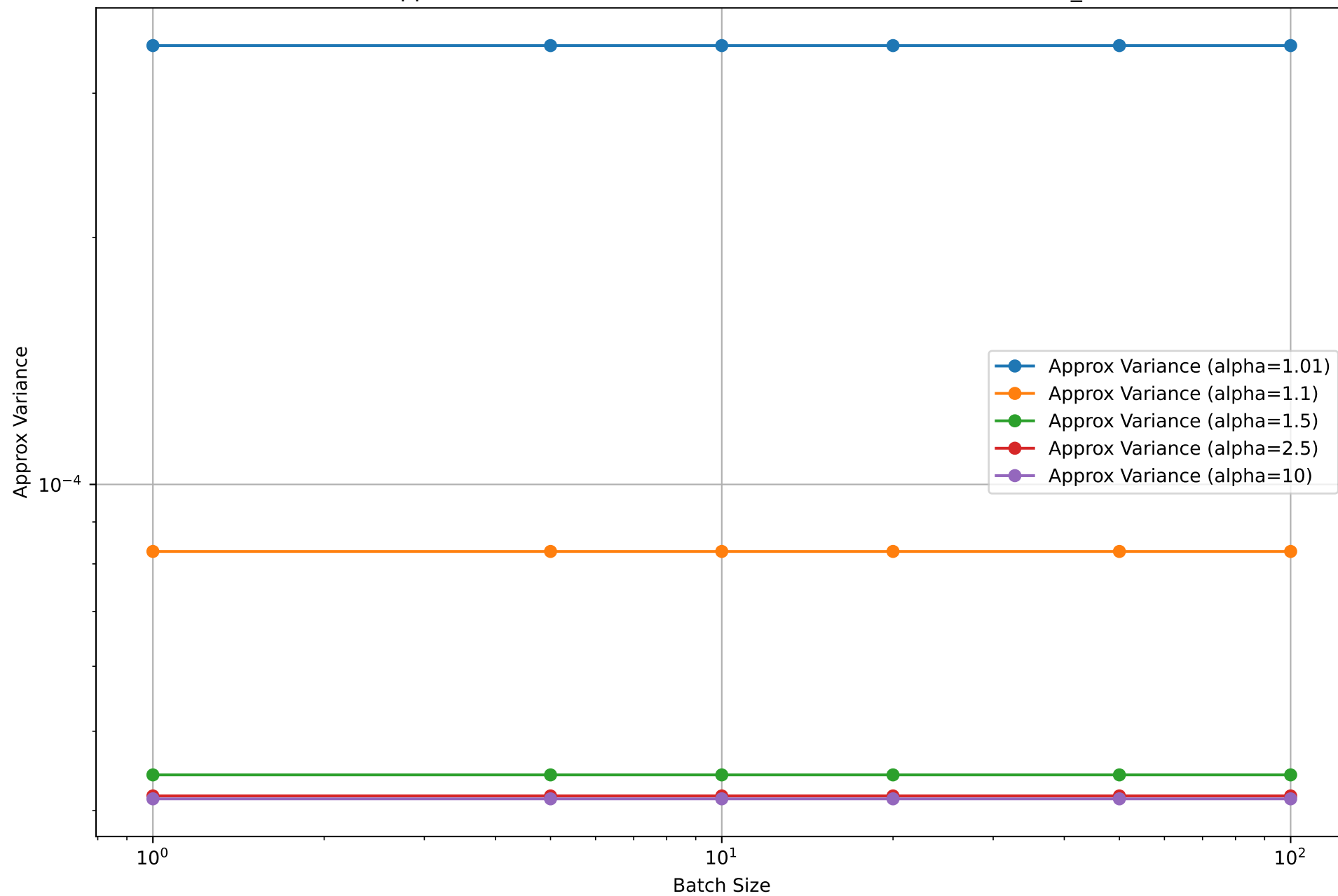
Slock Approx Variance for Different Batch Sizes; b \cdot T = 2000000 , \eta_{\text{star}}
