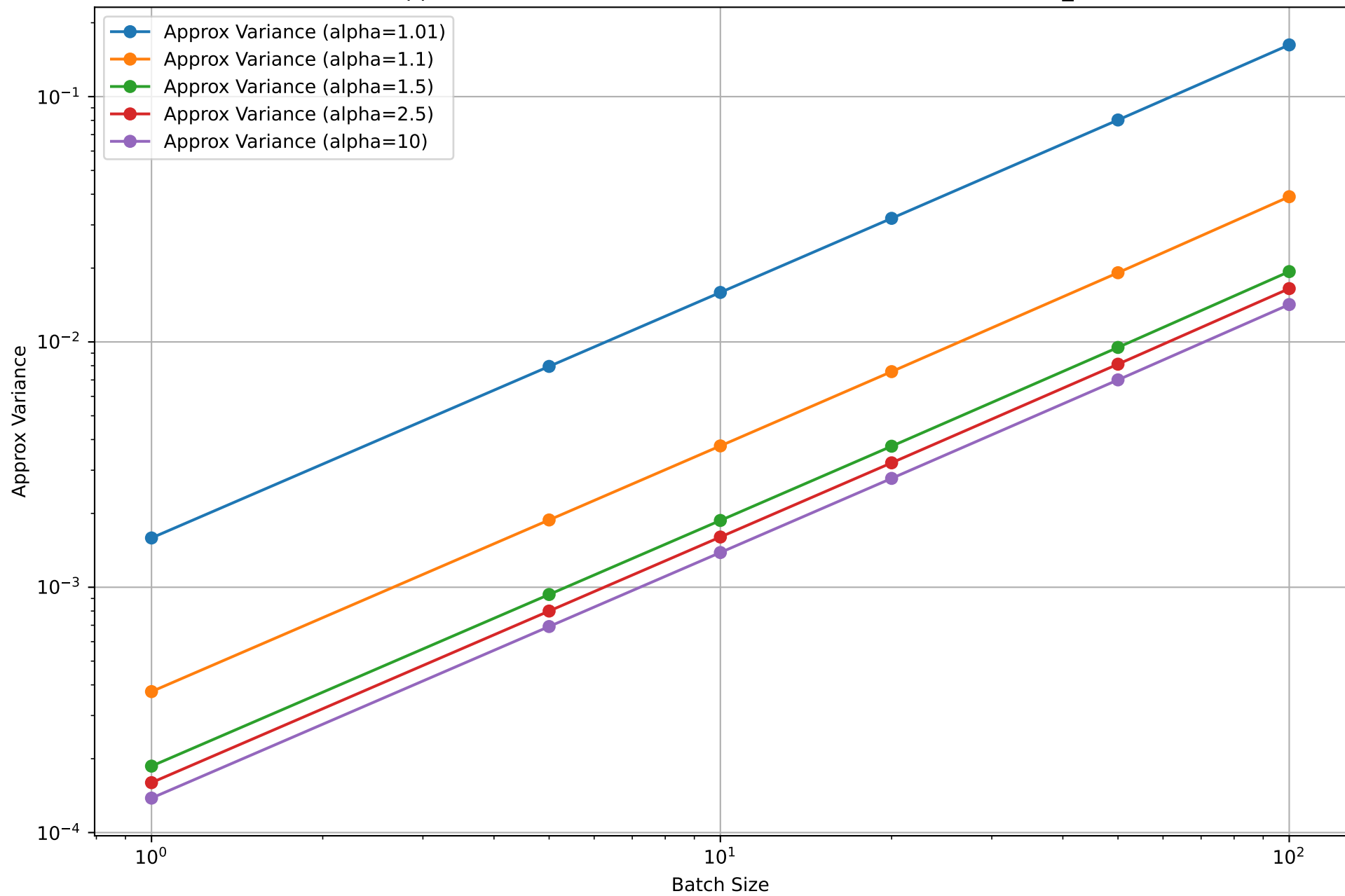
Slock Approx Variance for Different Batch Sizes; b \cdot T = 200000 , \eta_{\text{star}}
