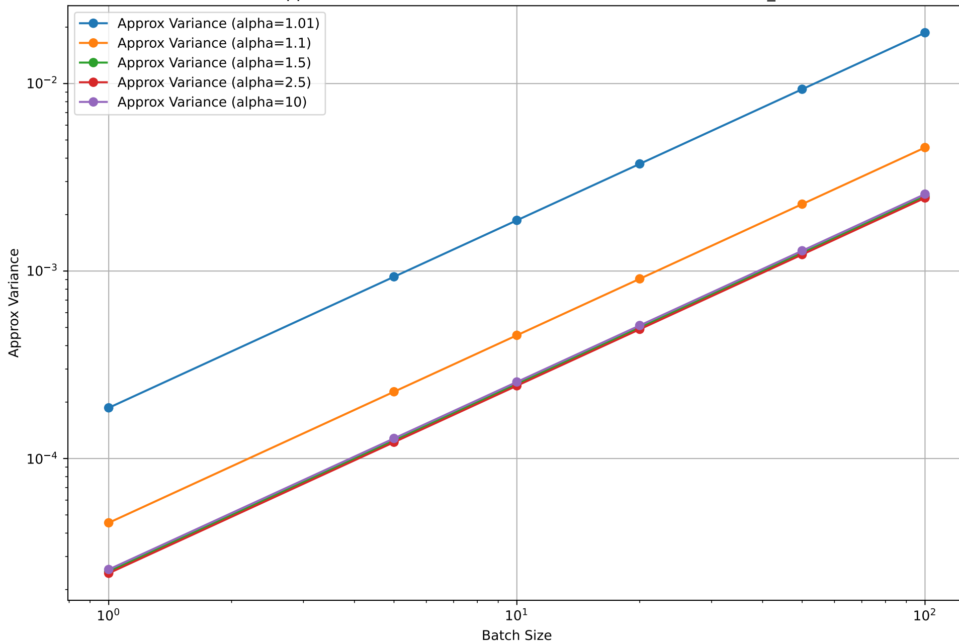
Slock Approx Variance for Different Batch Sizes; b \cdot T = 5000000 , \eta_{\text{star}}
