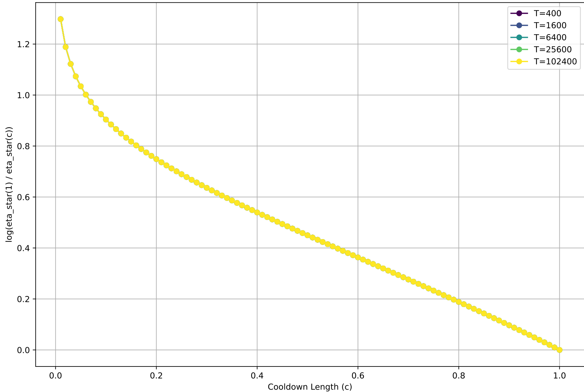
Effect of Cooldown Length on Optimal Learning Rate ( \eta_{\text{star}} ) for Different T
