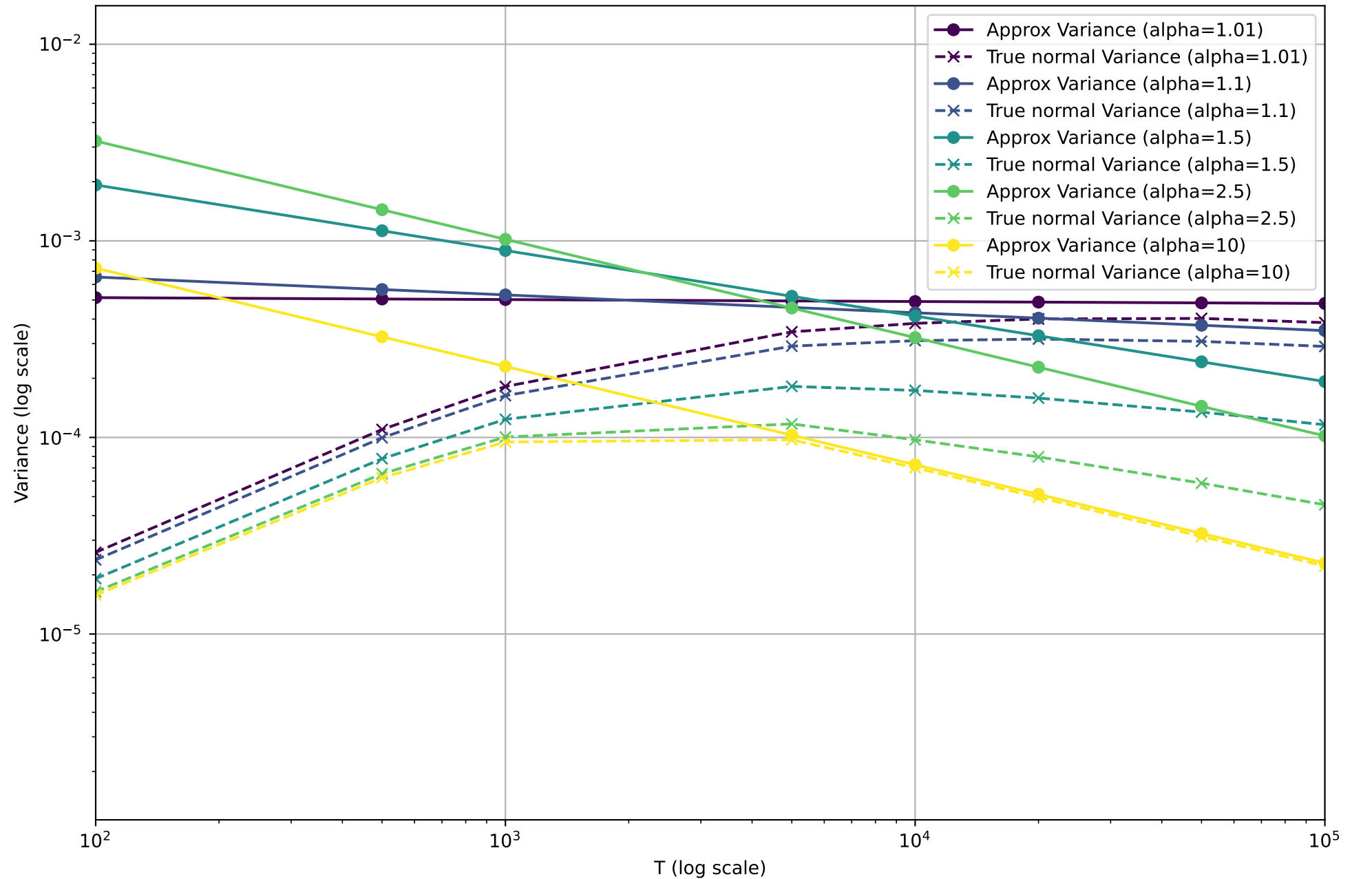
Variance Trajectories for Different Alphas (normal vs True) eta=0.001
