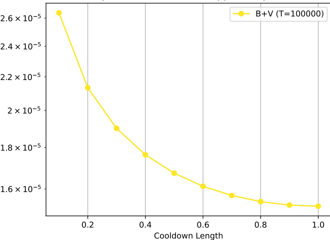
Risk optimized \eta^* (True vs Approx), \alpha=2.6
