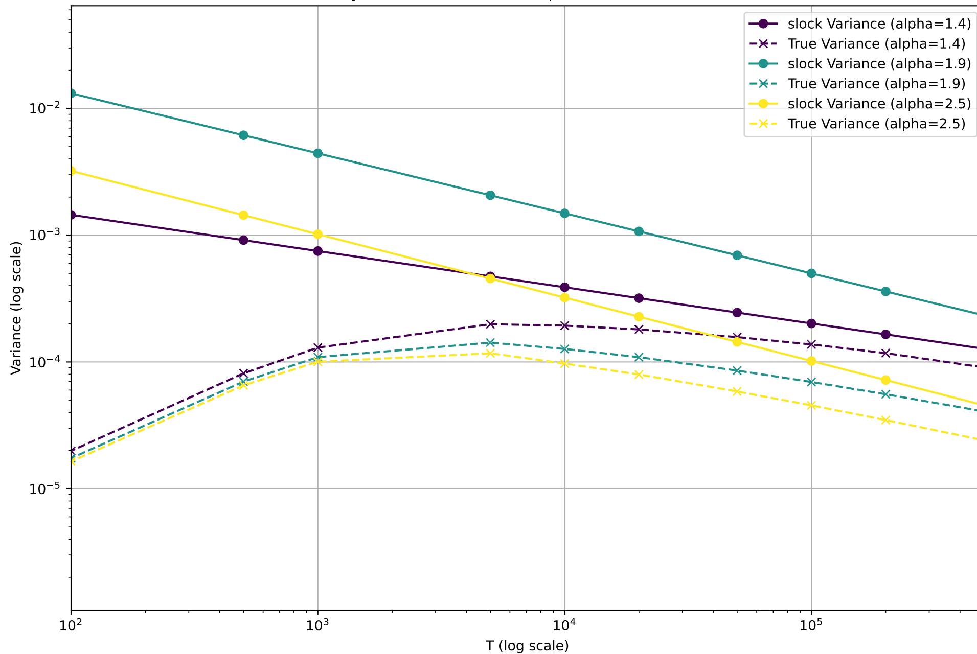
Variance Trajectories for Different Alphas (slock vs True) \eta=0.001
