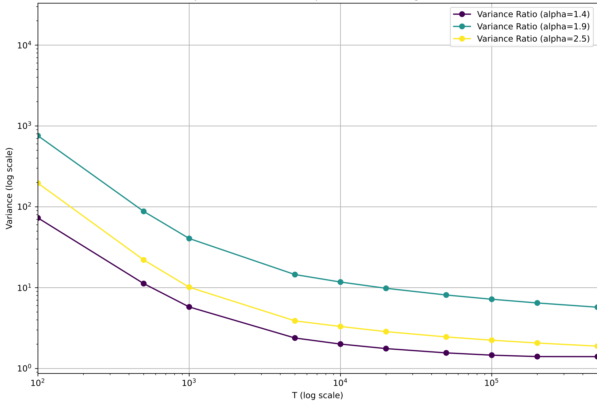
Variance Trajectories for Different Alphas (SLOCK vs Diagonal) \eta=0.001
