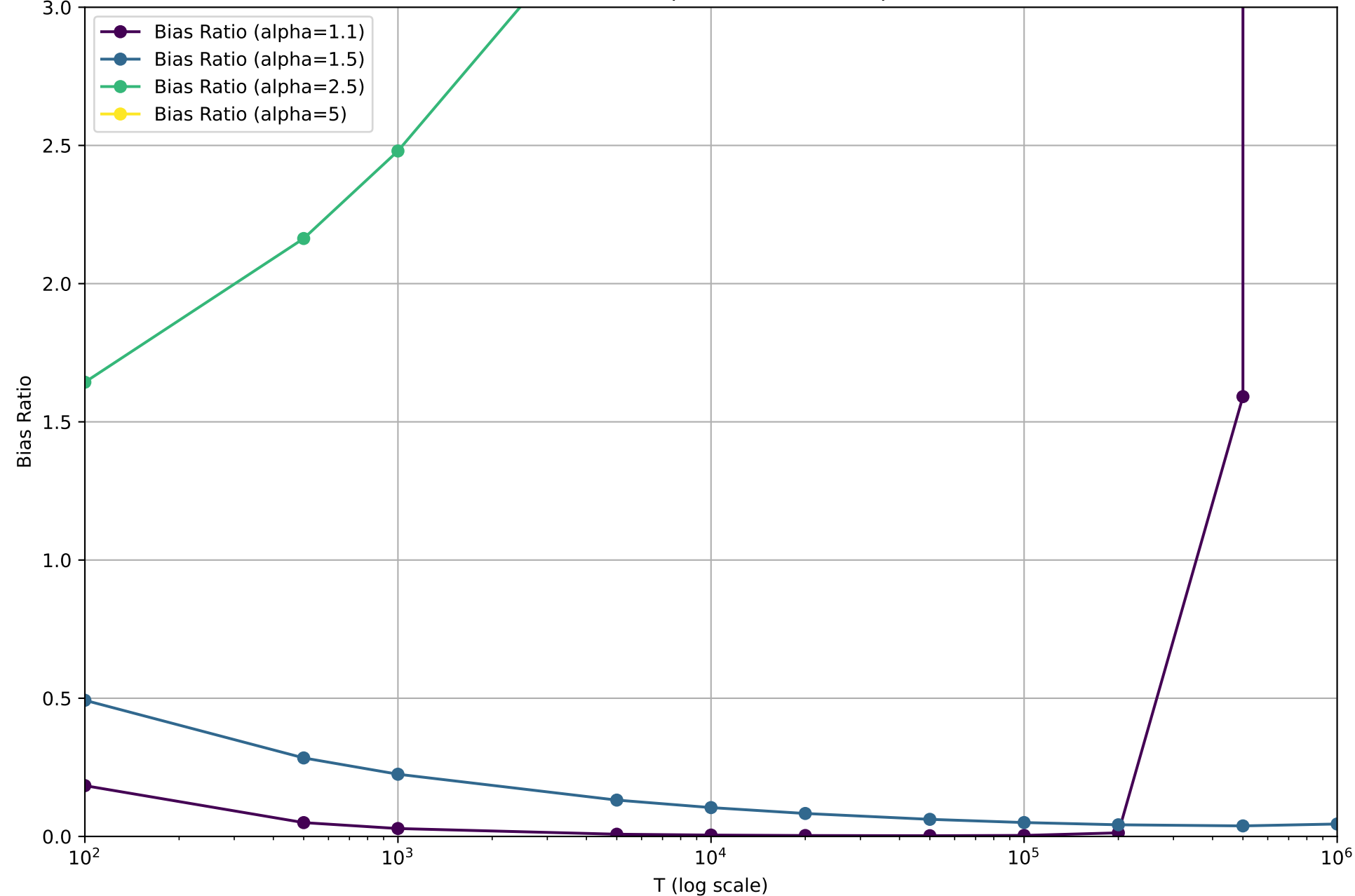
Bias Ratios for Different Alphas (SLOCK vs Laplace) eta=0.1
