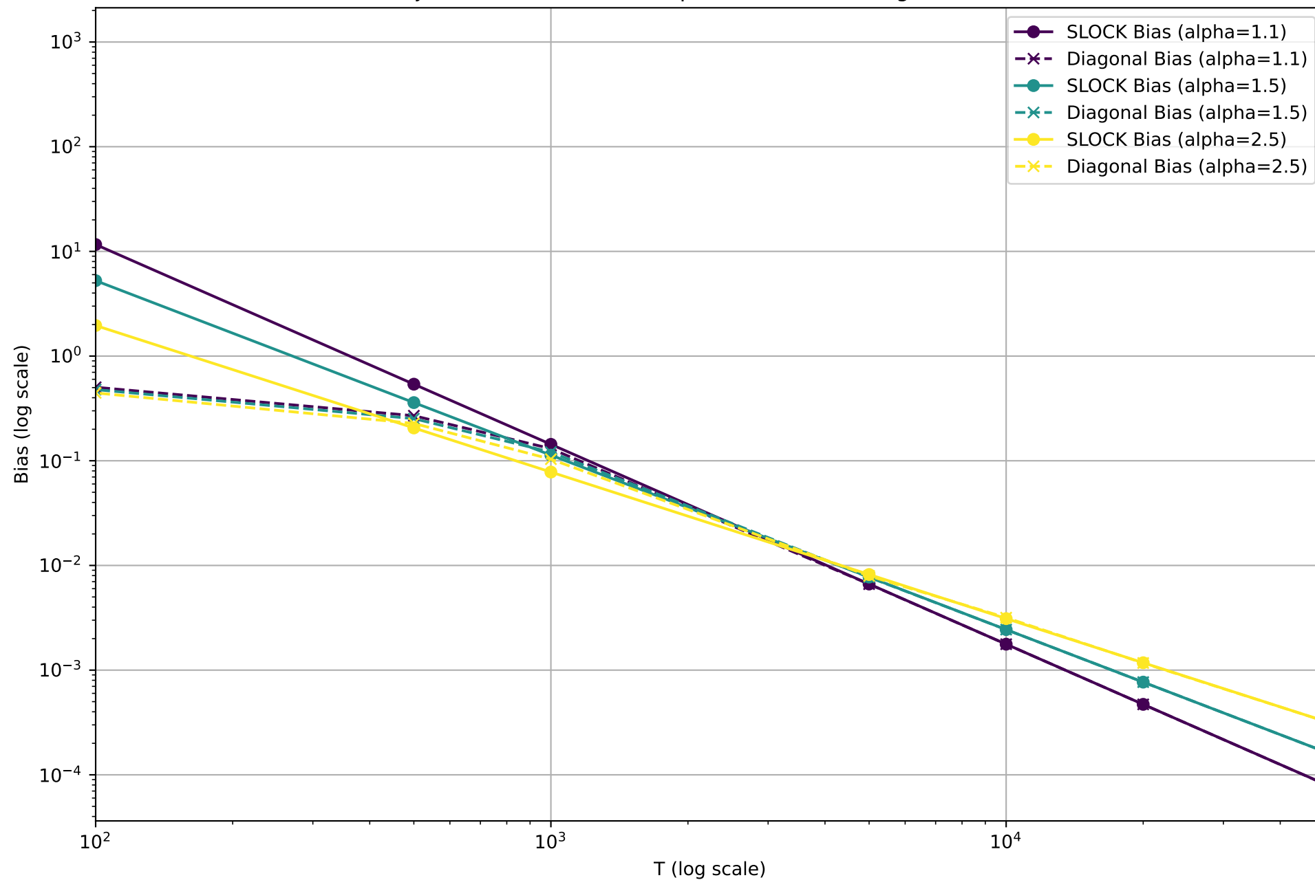
Bias Trajectories for Different Alphas (SLOCK vs Diagonal) \eta=0.001
