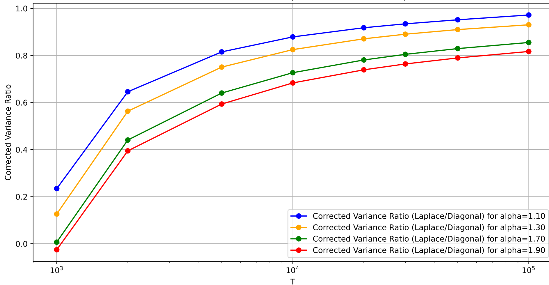
Corrected Variance Ratio Trajectories for Different Alphas
