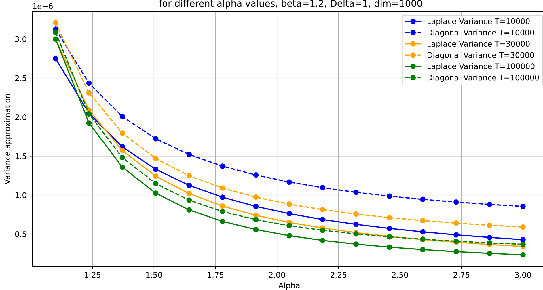
Variance of Laplace approximation vs Diagonal approximation for linear schedule at K=1 for different alpha values, beta=1.2, Delta=1, dim=1000
