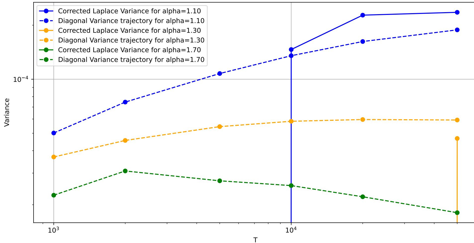
Corrected Variance Trajectories for Different Alphas, 100
