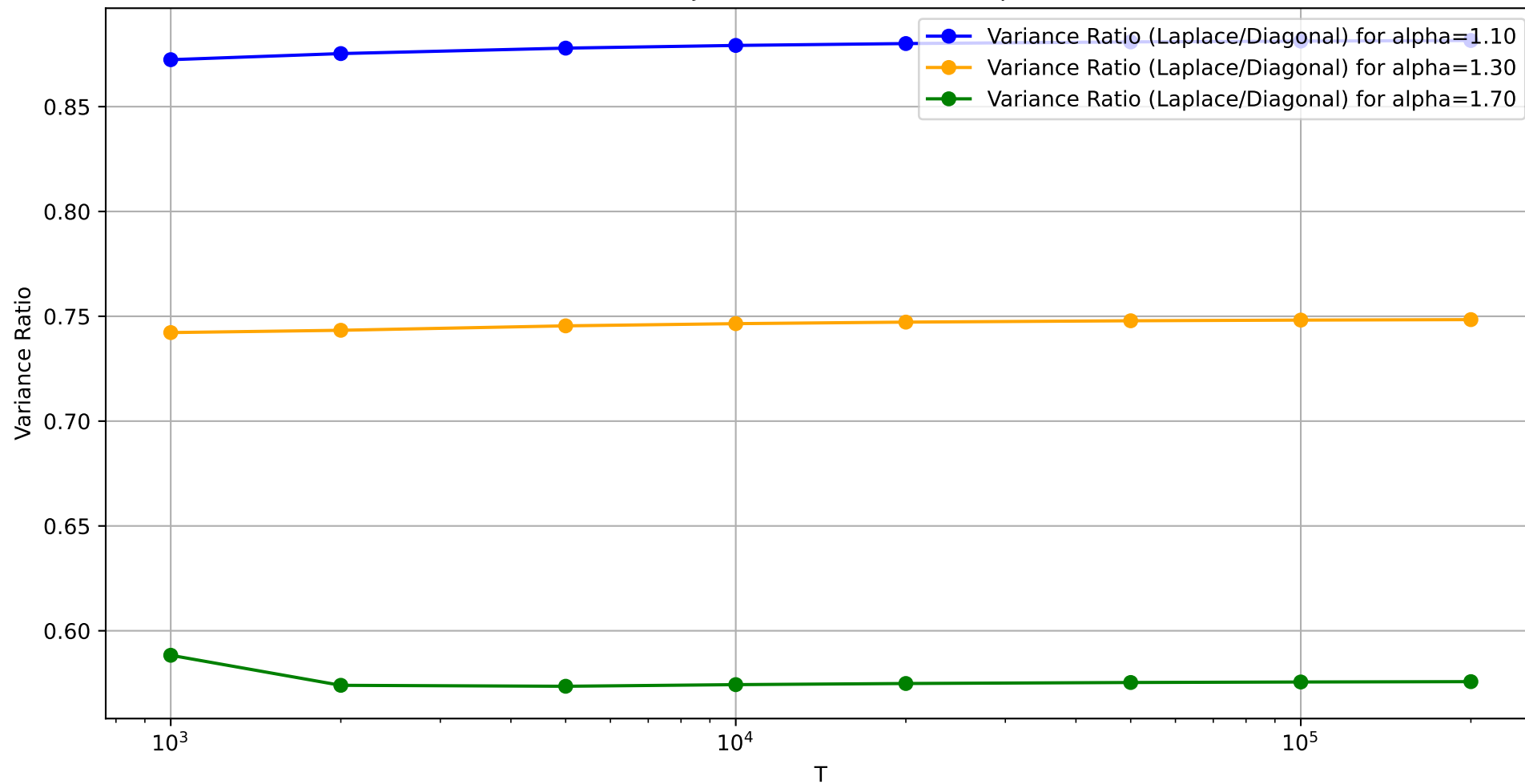
Variance Ratio Trajectories for Different Alphas, dim=10
