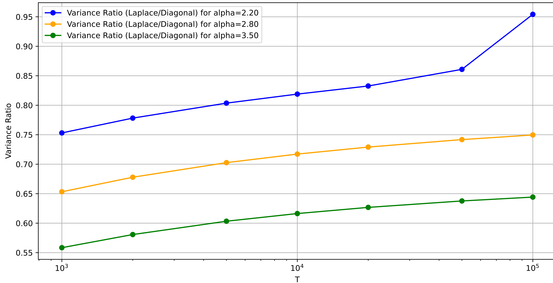
Variance Ratio Trajectories for Different Alphas, dim=100
