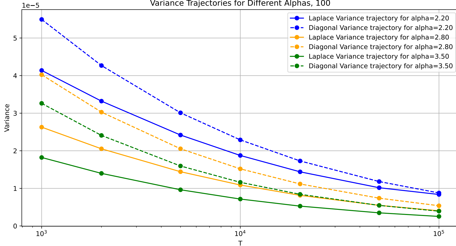
Variance Trajectories for Different Alphas, 100
